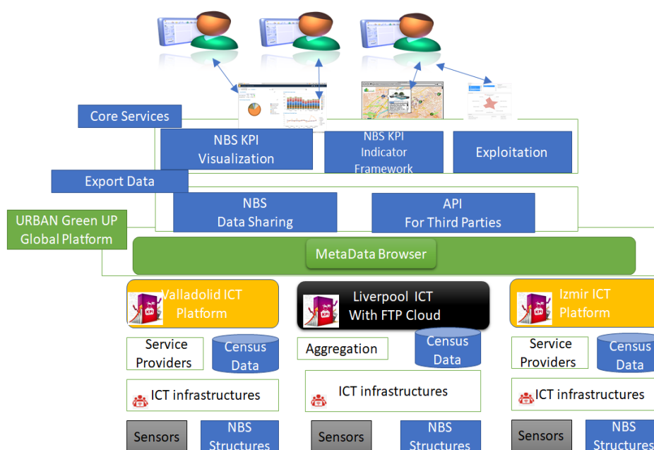
Figure 4.5: ICT platform diagram II
