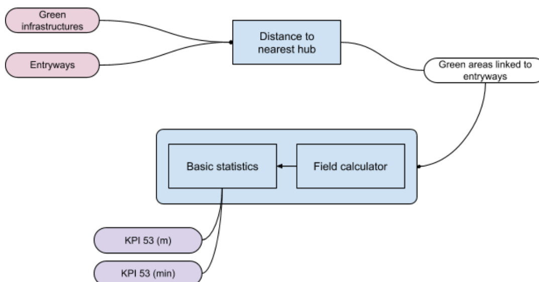
Figure 2.6 Algorithm for this described process
