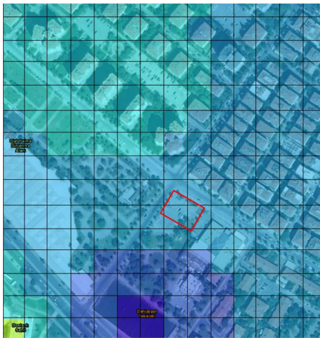
Figure 2-7 Landsat-8 LST 30 m grid overlapped with high-resolution image – Study area 2
