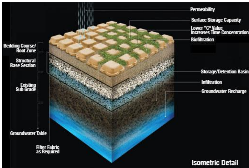
Figure 2-10: A detailed figure of pavement product 2
