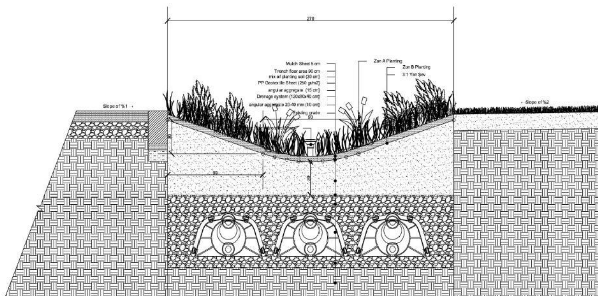
Figure 3-8: Section of Bioswale
