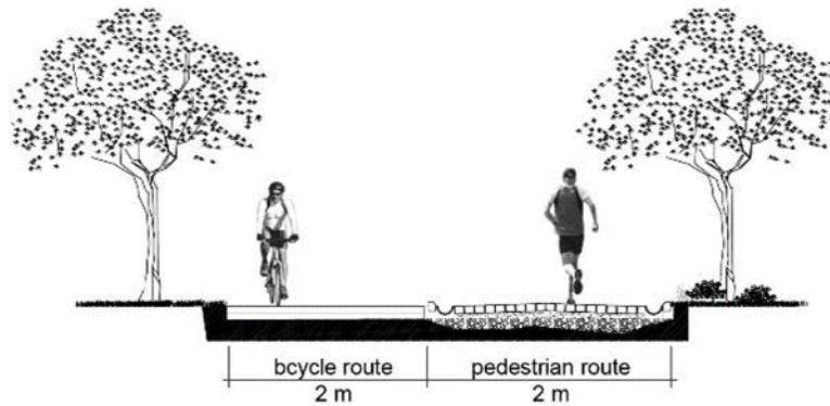
Figure 4-4: Schematic view of cycle and pedestrian route
