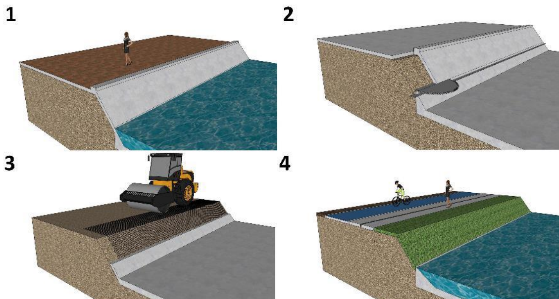
Figure 4-5: Schematic view of culvert works in Peynircioğlu Stream
