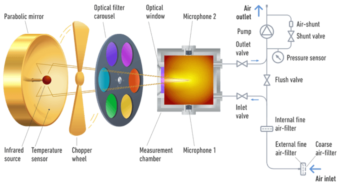
Figure 3-4: Schematic view of Photoacoustic Gas Monitor instrument
