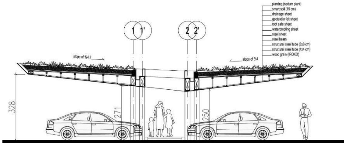
Figure 2-12: Green Covering Shelter for car park section
