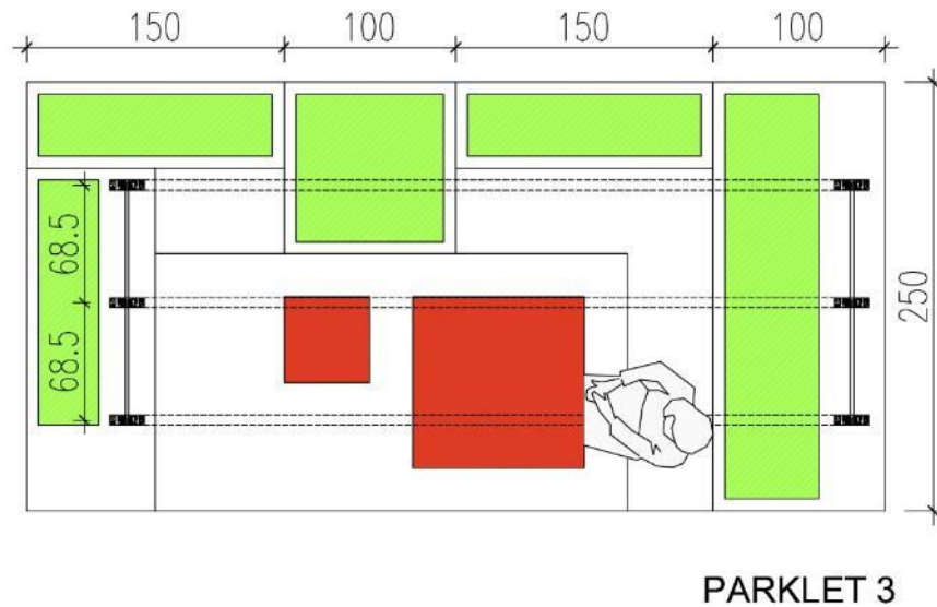
Figure 2-7: Technical Drawing of Parklet #3
