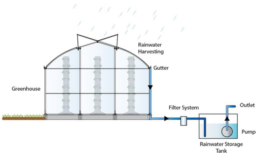
Figure 3-13: Schematic view of rainfall harvesting
