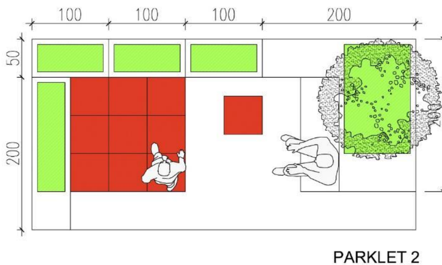
Figure 2-6: Technical Drawing of Parklet #2
