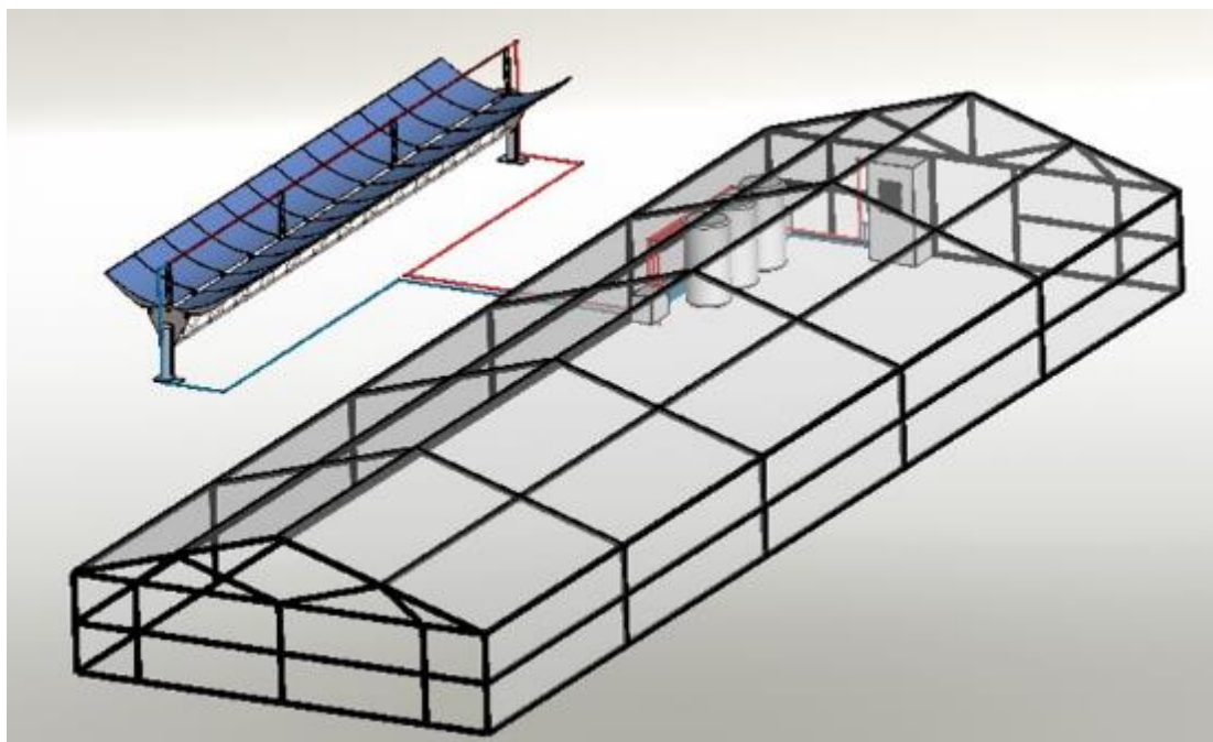
Figure 3-15: Schematic view of parabolic type solar energy collector
