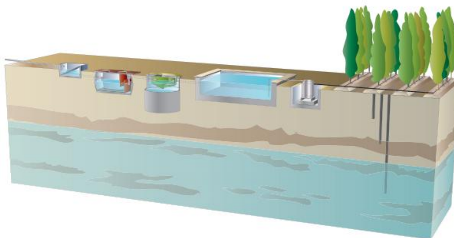
Figure 4.28: Typical flow-sheet of a Green Filter or Land application system
