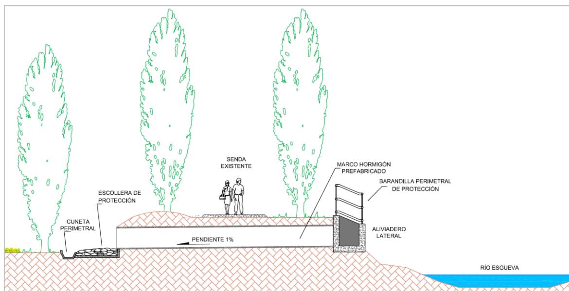
Figure 4.53: Schematic preliminary design for the waterflow inlet control structure
