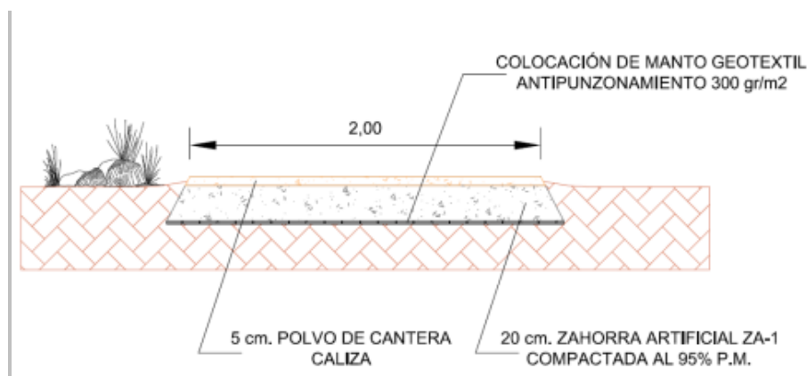
Figure 4.75. Transversal section for the Educational Path (Source: River Duero Basin)
