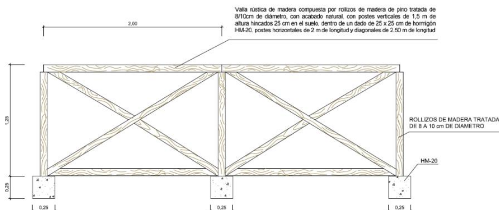
Figure 4.87. Suggested design for security barriers
