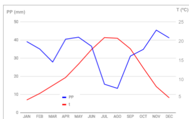
Figure 4.59: Climodiagram, Valladolid
