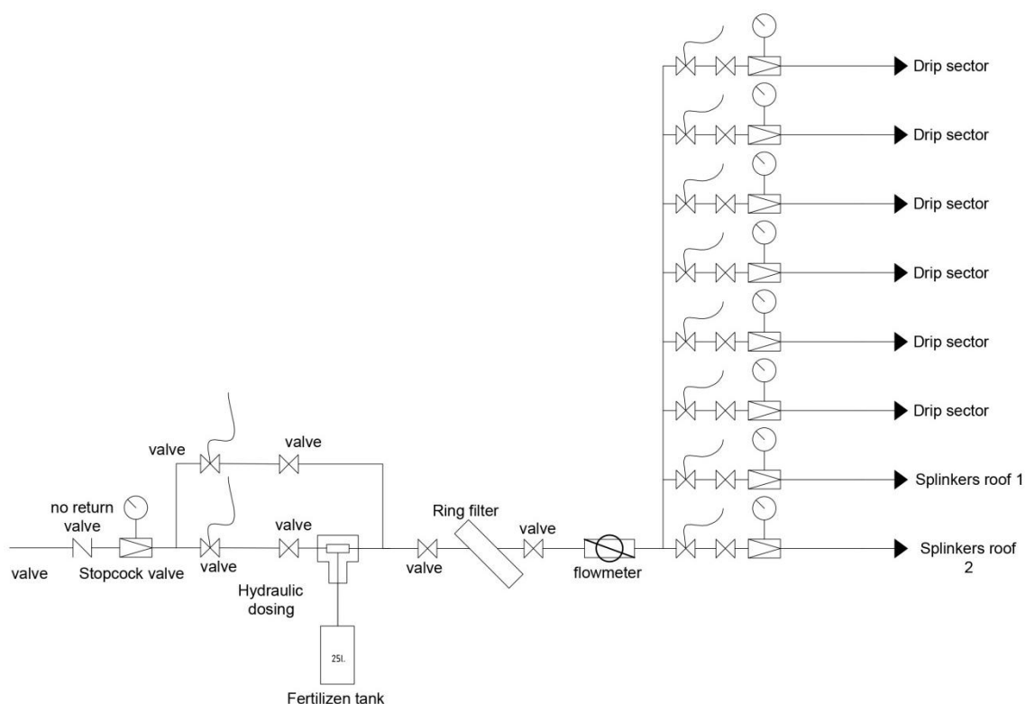
Figure 3.32: Green Covering Shelter irrigation scheme
