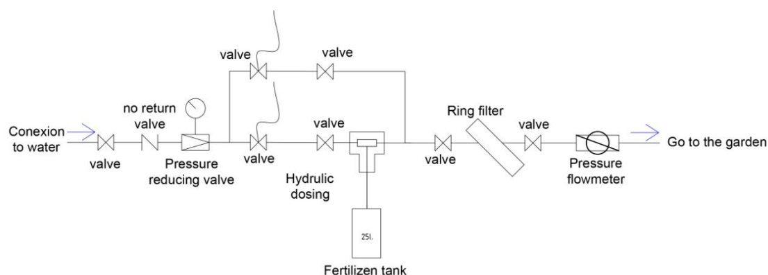
Figure 3.16: Irrigation scheme of Vertical mobile gardens.
