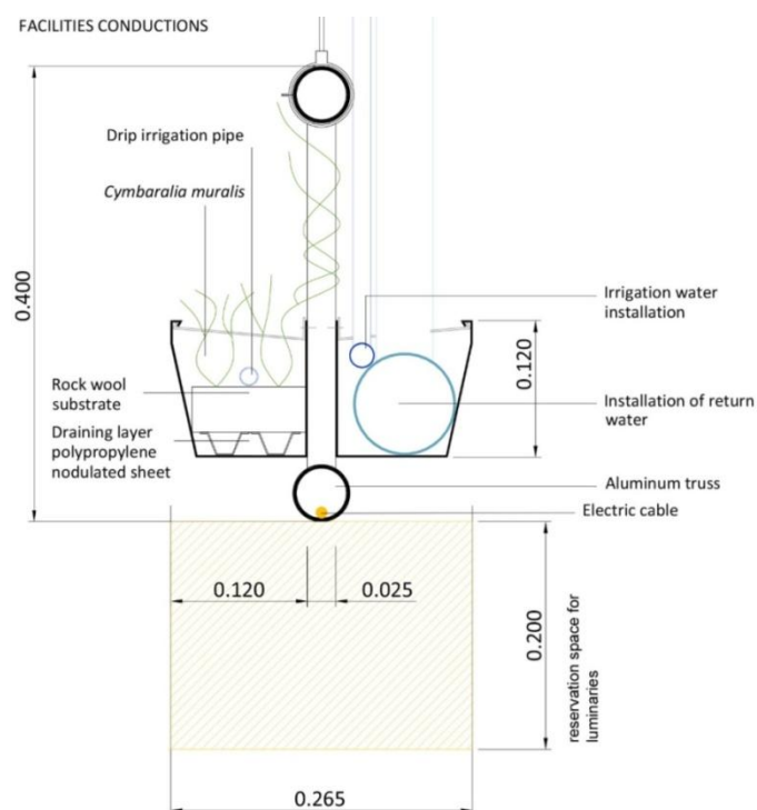
Figure 3.45: Detail of facilities ducts - Green Shady Structures
