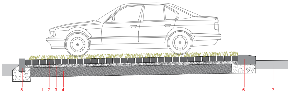
Figure 4.5: Technical section of the green parking pavement
