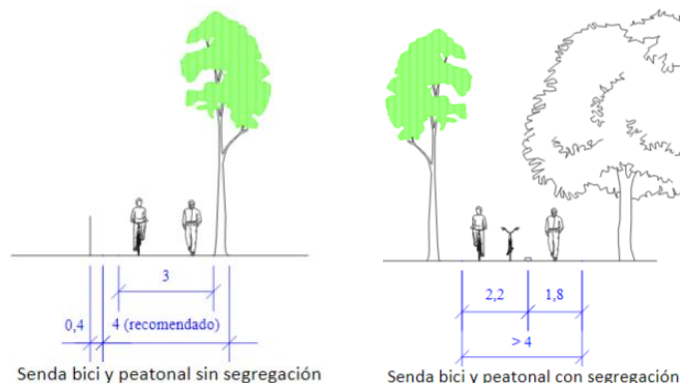
Figure 2.10: Cycle-path section (Source: revision PGOU 2017)
