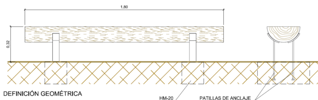
Figure 4.82. Alternative design for rustic rest benches
