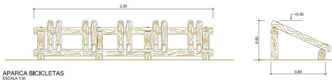
Figure 4.85. Suggested design for rustic parking area for bicycles
