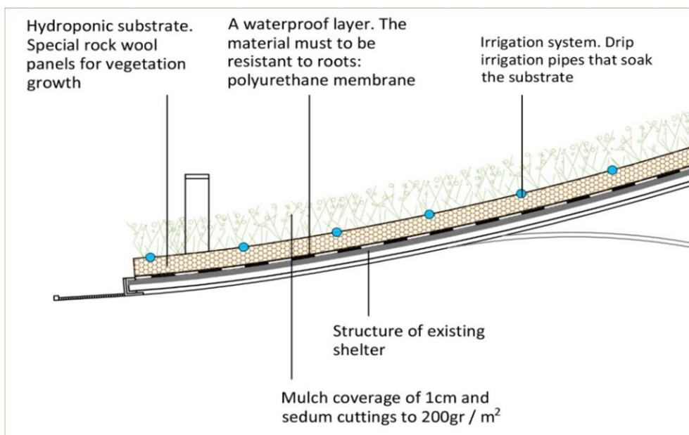
Figure 3.31: Detail of the Green Covering shelter design
