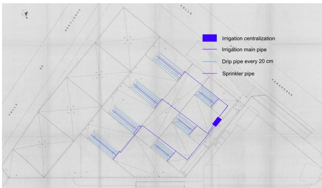
Figure 3.37: Pipe distribution of the Green Roof.
