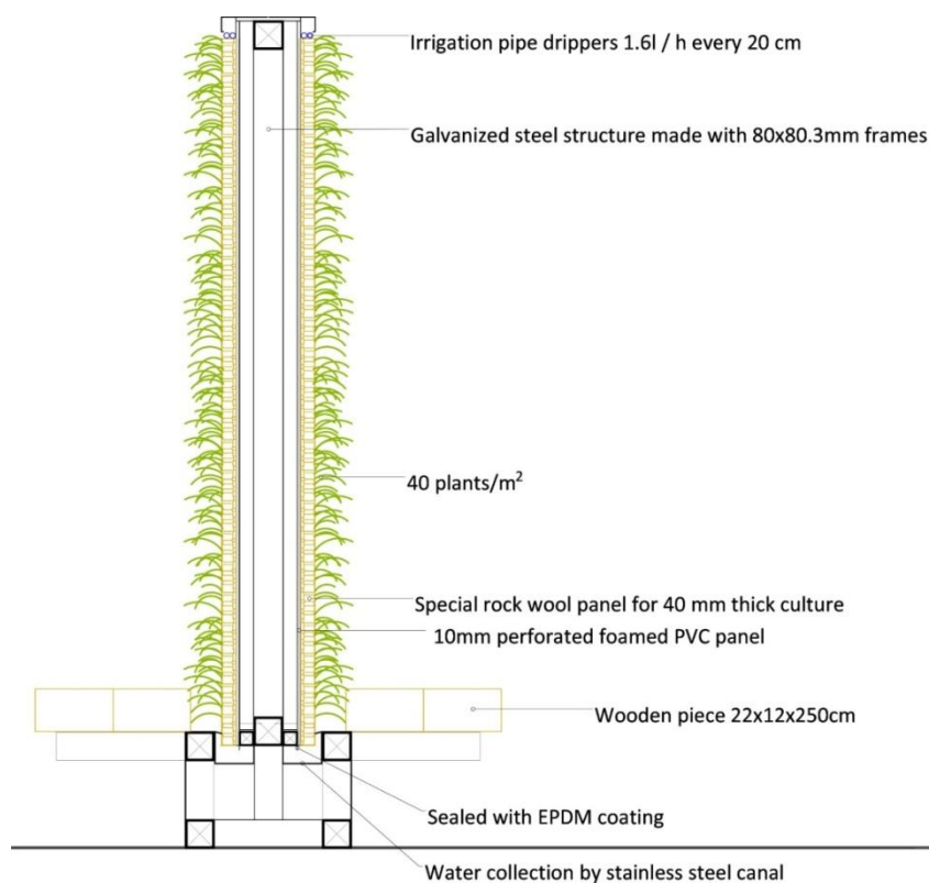
Figure 3.14: Vegetable board constructive section.
