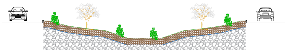
Figure 4.12: Section of the detention basin
