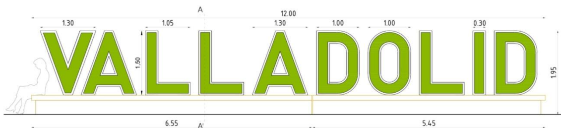
Figure 3.8: Vertical mobile garden - Elevation of vegetable sculpture
