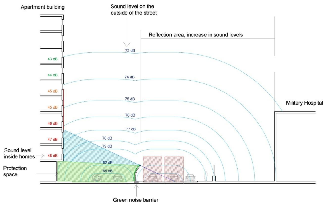
Figure 3.3: Noise scheme for the Paseo Hospital Militar street section (Green noise barriers)
