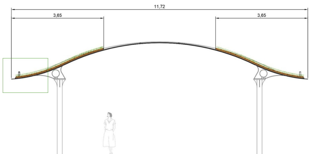
Figure 3.30: Elevation of the Plaza España green covering shelter
