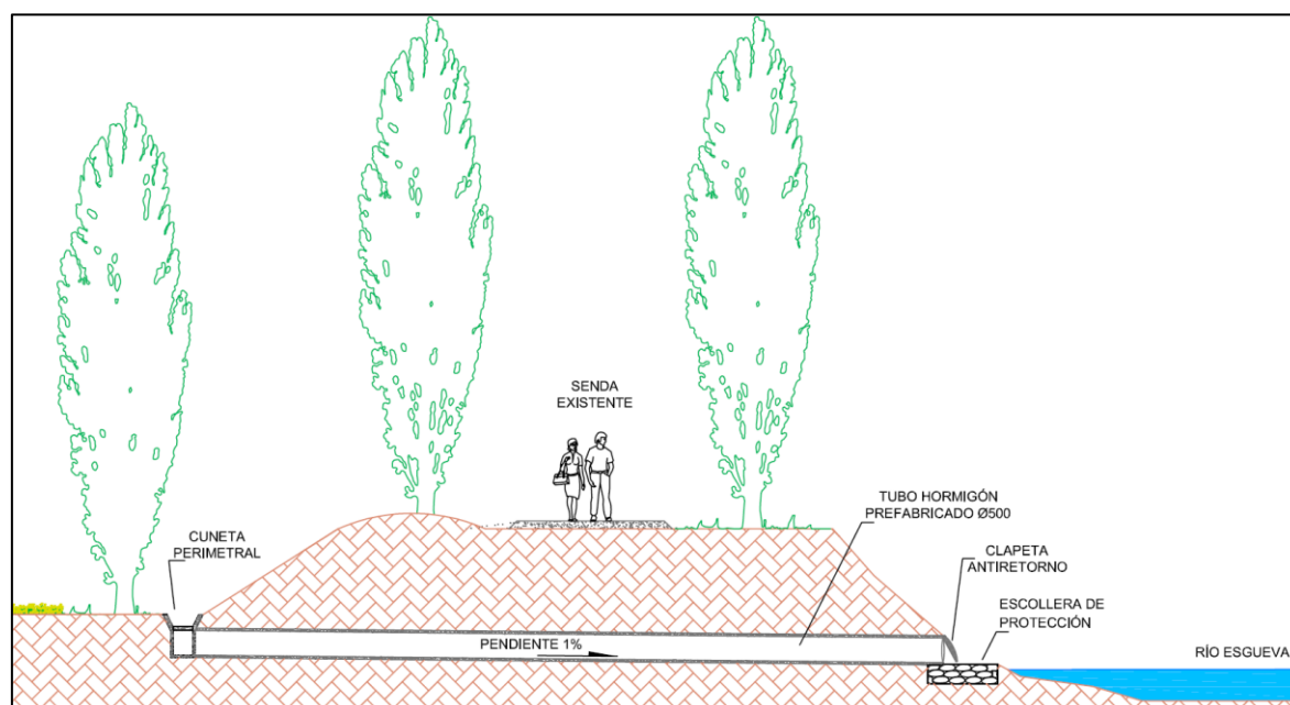
Figure 4.55: Schematic preliminary design for the waterflow outlet control structure.
