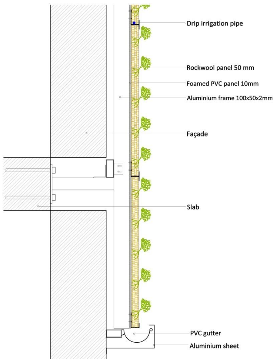
Figure 3.26: Constructive section of the vertical garden - Green façade in the Corte Inglés.
