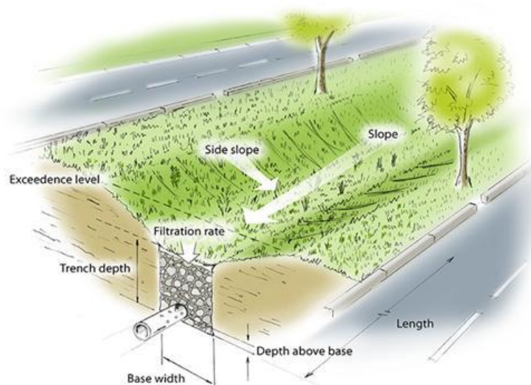
Figure 2.49: Green swale scheme (SUD)
