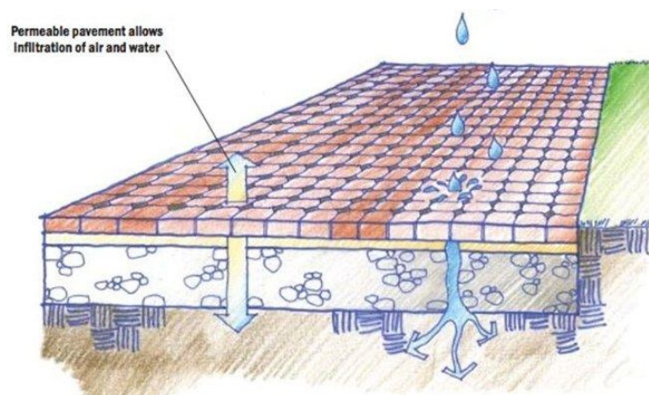
Figure 2.33: Permeable pavements (Source: organicsolutions.com)
