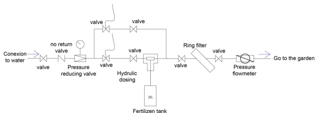
Figure 3.7: Irrigation scheme of Green Noise Barriers
