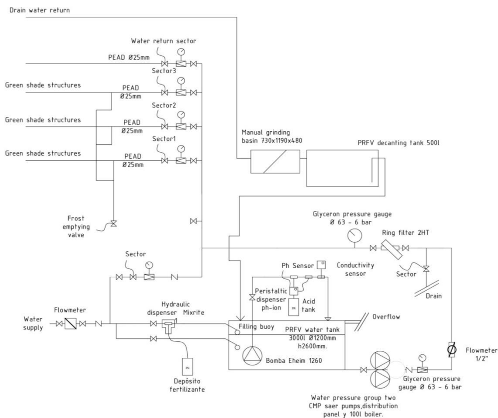
Figure 3.46: Irrigation scheme - Green Shady Structures
