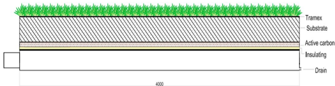
Figure 3.56. Urban Garden Bio-Filter front view
