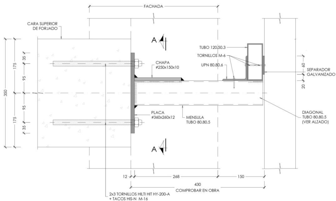
Figure 3.23: Moorings to the slabs - Green façade in the Corte Inglés
