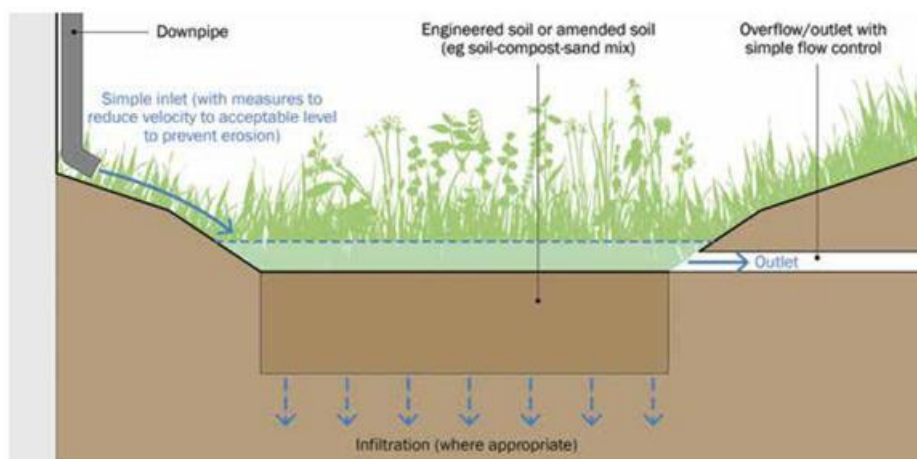
Figure 2.51: Rain garden scheme (SUD)
