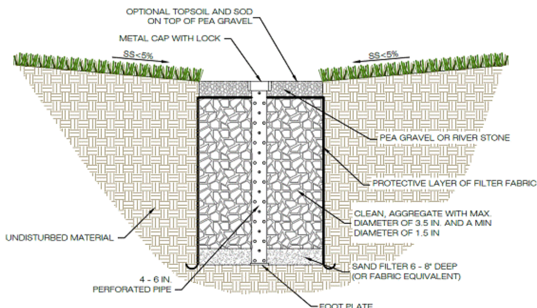
Figure 4.13: Section of the infiltration well
