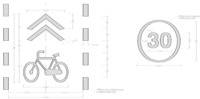
Figure 2.19: Horizontal signalling for cycle tracks (Sp. Ciclo-calle and Zona 30 . Source: Junta de Andalucía)
