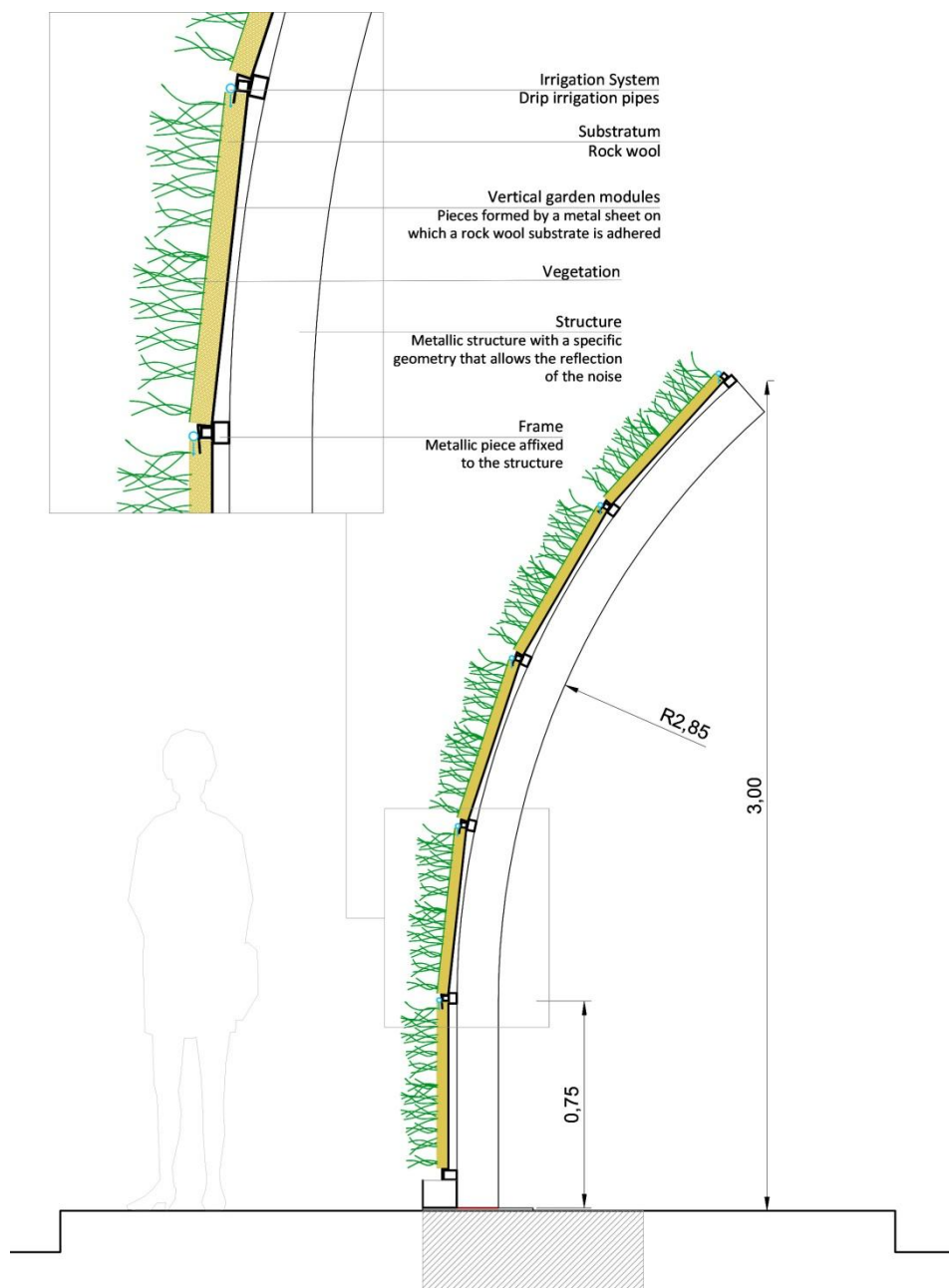
Figure 3.6: Constructive section of the Green Noise Barriers
