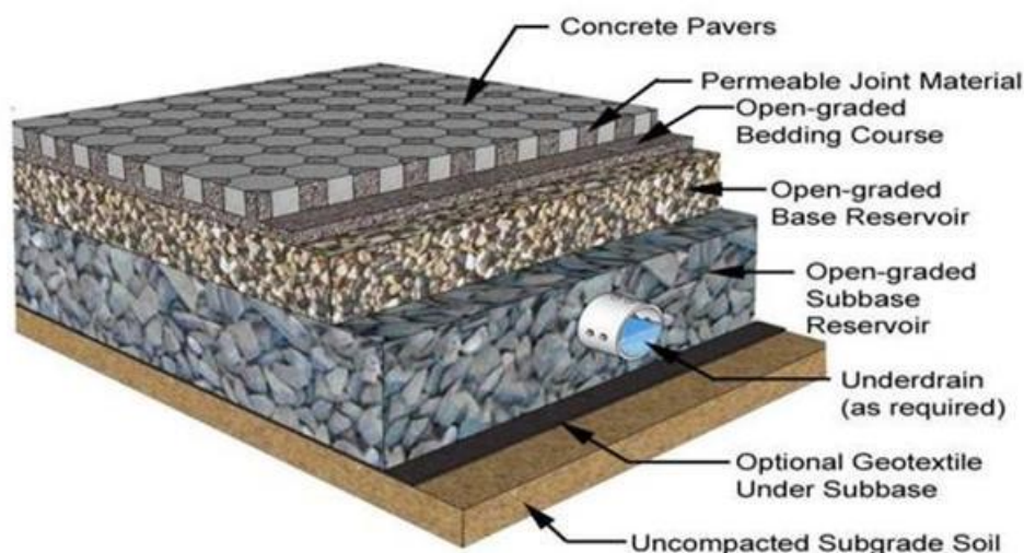
Figure 2.47: Filtering pavement layers (SUD)
