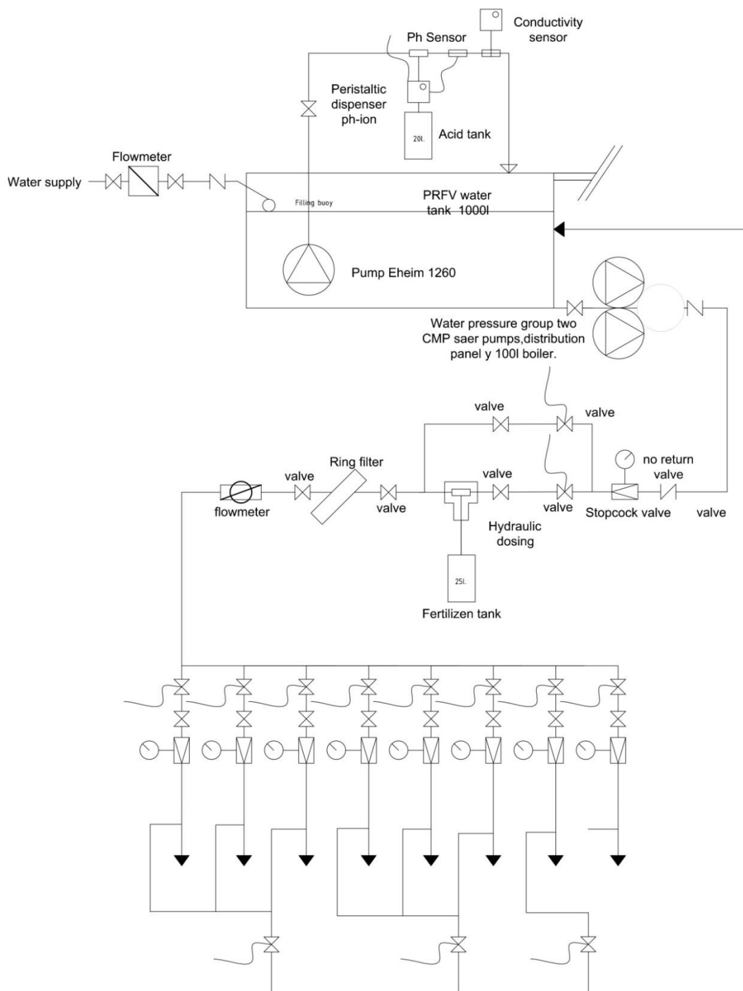
Figure 3.27: Irrigation scheme - Green facade in the Corte Inglés.
