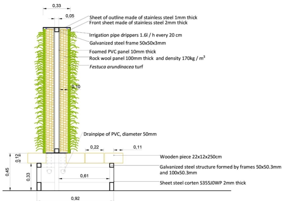
Figure 3.13: Vegetable sculpture constructive section.
