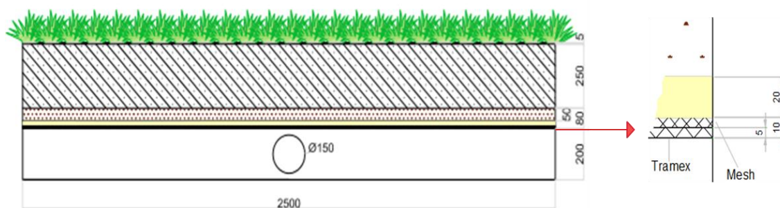
Figure 3.57. Urban Garden Bio-Filter side view
