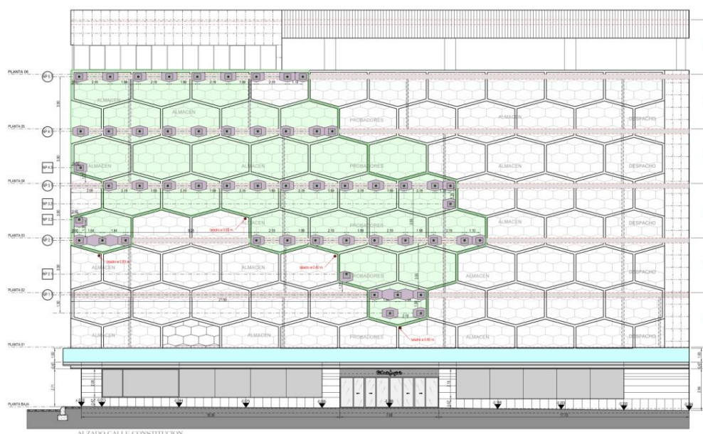
Figure 3.21: Clamping structure on the north façade - Green facade in the Corte Inglés
