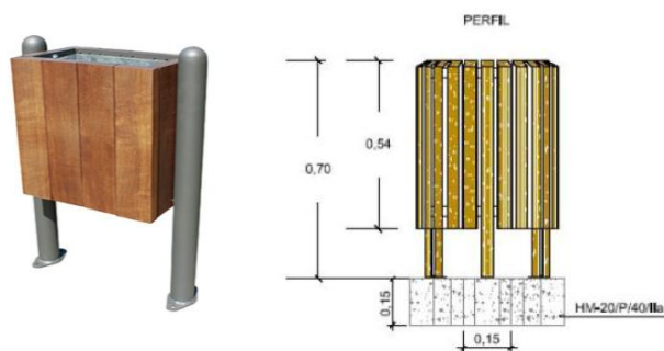
Figure 4.80. Suggested design for waste bin (overturned mode)
