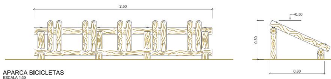
Figure 2.27. Suggested design for rustic bicycles parking areas
