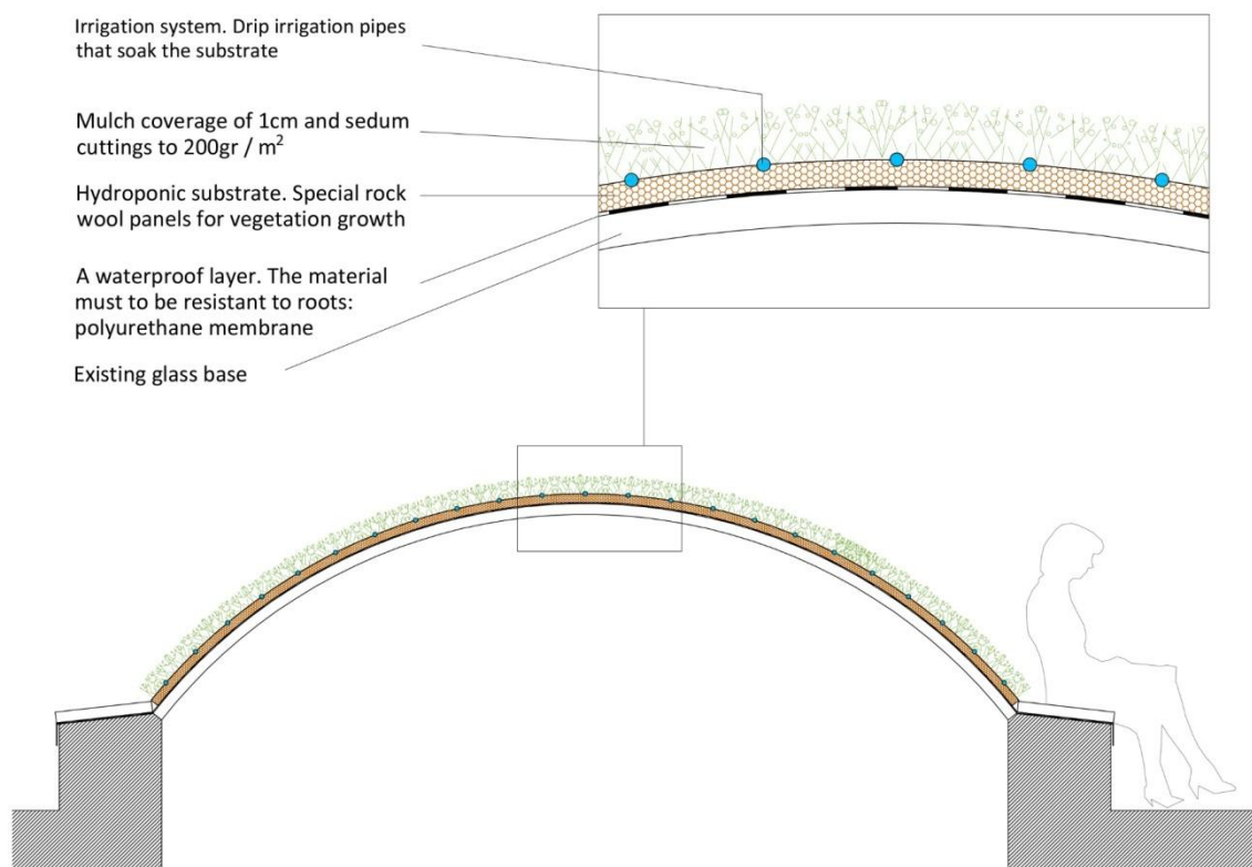
Figure 3.36: Technical detail of the Green Roof.
