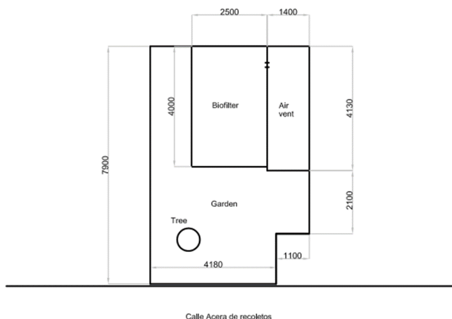
Figure 3.58. Urban Garden Bio-Filter top view.
