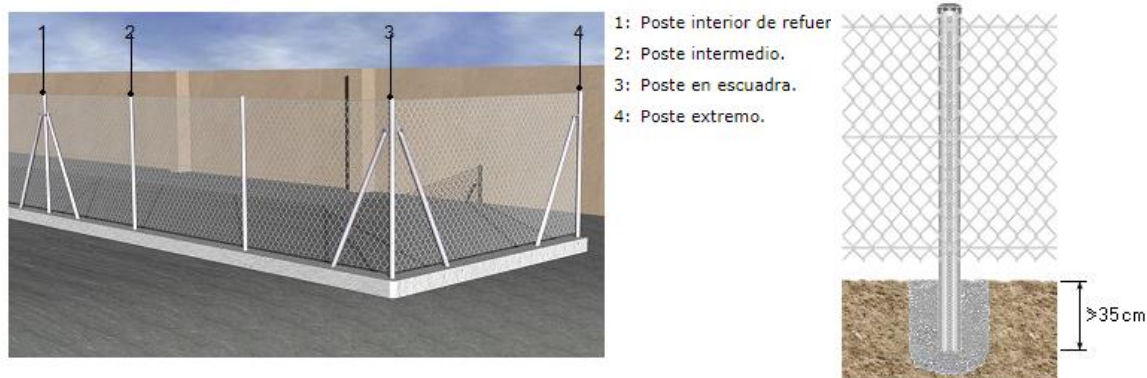
Figure 4.56: Suggested design of the perimeter fence
