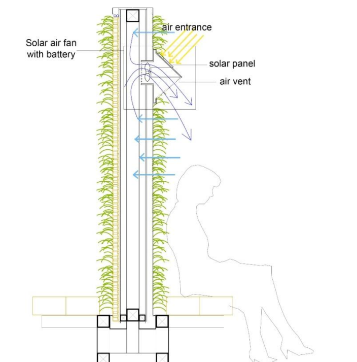
Figure 3.14: Vegetable board constructive section.
