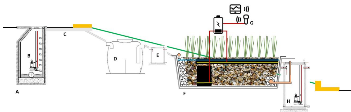
Figure 3.50: Scheme of the treatment line of the Electrowetland.
