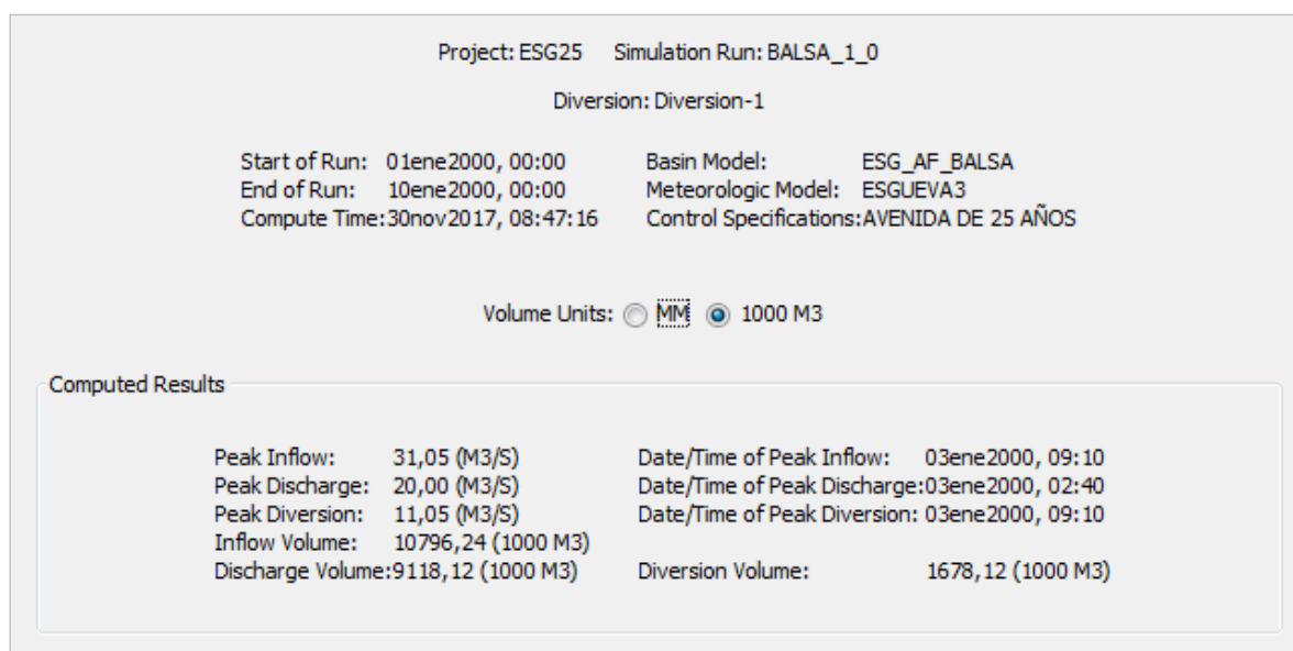
Figure 4.40: Hydrological model results (return period = 25 years)
