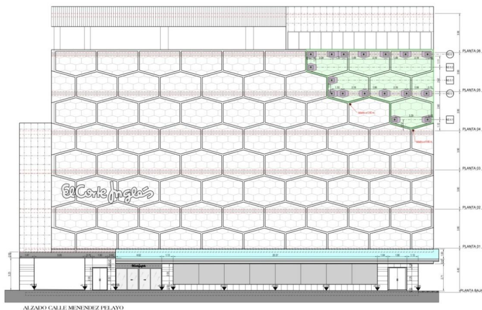
Figure 3.22: Camping structure on the east facade - Green facade in the Corte Inglés
