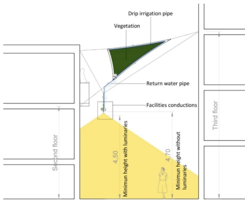
Figure 3.44: General section - Green Shady Structures
