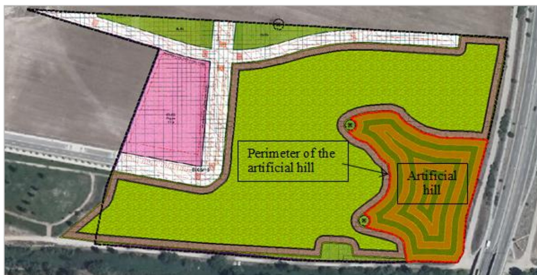
Figure 4.52: Preliminary design of the artificial hill.
