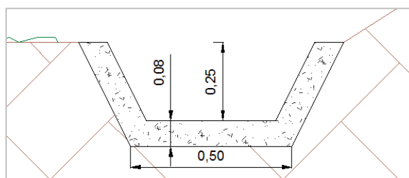
Figure 4.51: Preliminary design of the perimeter ditch section.
