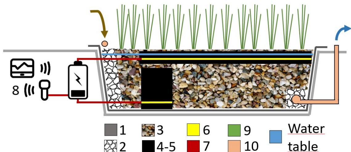
Figure 3.49: Conceptual drawing of an Electrowetland.
