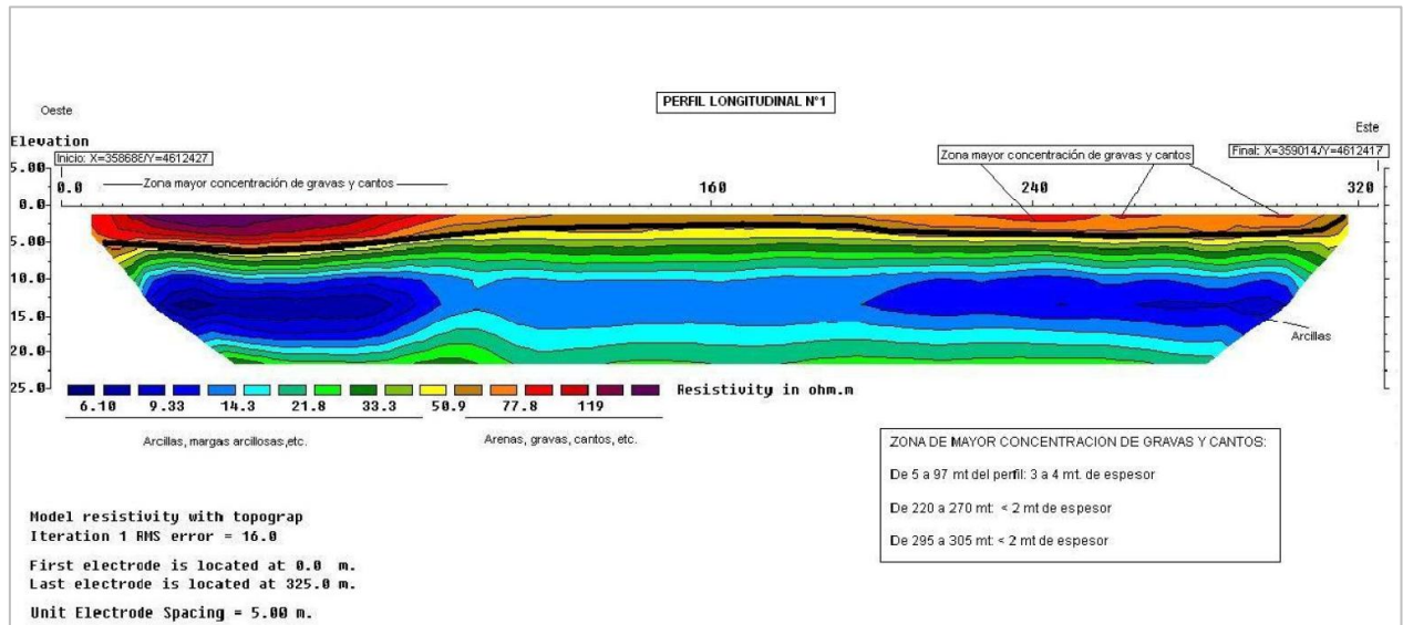
Figure 4.49: Example of the results obtained from the longitudinal profile nº1 of the Electrical Tomography
